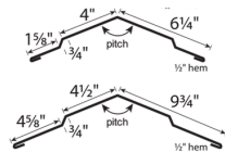
RIDGE CAP
