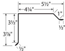
RESIDENTIAL RAKE
