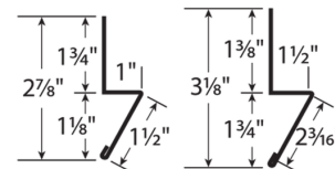
RAT GUARD
