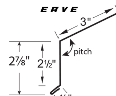
EAVE
