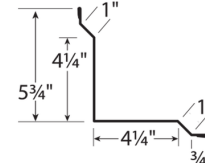
INSIDE CORNER
