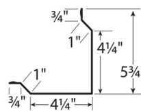
RAKE & CORNER
