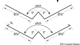
VALLEY
